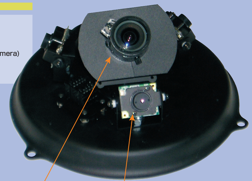
Supplemental camera * Wide angle lens & High-Quality color camera. * Available in Standard and High-Resolution. Main camera * Can choose various lenses Fixed/Variable Focal Auto Iris/Variable focal day/night.
